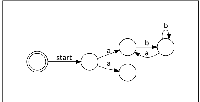
Figure 4.5. FSCA FSM diagram generated by the tool with unreachable states
